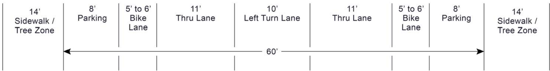
MARYLAND AVENUE NE PROPOSED ROADWAY SECTION WITH 10' LEFT TURN LANE
